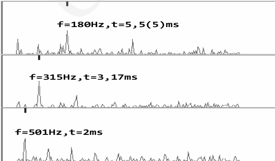
Fig. 4. Cepstrums of the frames t_1 , t_2 , t_3 of the source signal. The X-axis is the time from the range (0.23)ms. (23.46)ms range is a mirror reflection due to the Fourier property and thus it is not depicted in the graph
