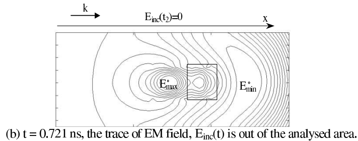
Fig. 5. Some snapshots of the propagated electromagnetic wave E_z(t) (the increment \Delta E_z of the isolevels is 0.0625 \text{ V/m} )
