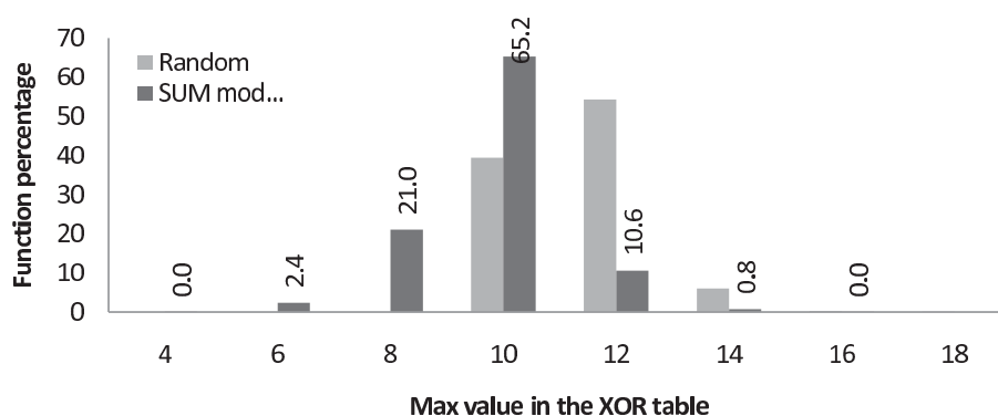
Fig. 12. Nonlinearity of S-boxes combined with a key using SUM mod 256.
